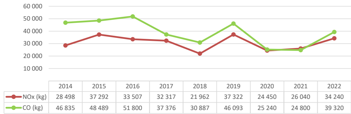
Figure 4.3 NO x , CO total emissions from Ispra trigeneration plant
