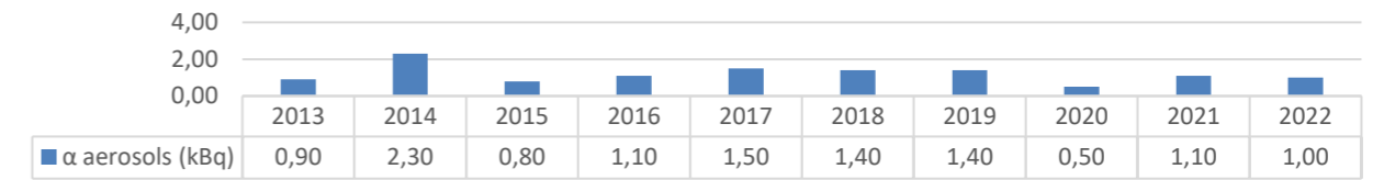
Figure 4.5 Atmospheric emissions containing α emitting aerosols at JRC Geel
